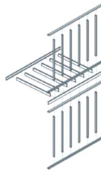
Stick-built
